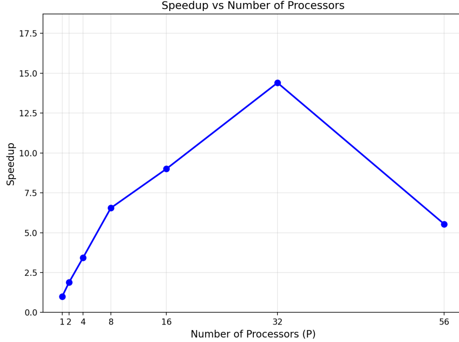
Figure 18: Speedup S(P) = T(1)/T(P) vs. number of processors P .
